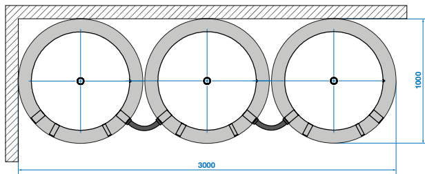
Parallel connection
